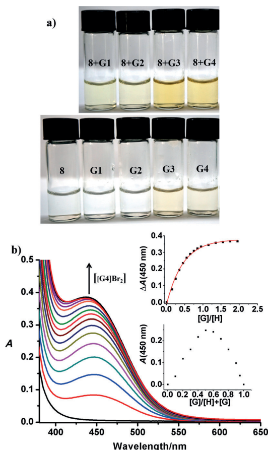
Figure 3. a) Color change after mixing host 8 with G1 – G4 in water. b) UV/Vis titration spectra at 20°C of 8 (0.8 mmol L −1 ) with addition of 0–1.95 equiv of G4 (from bottom to top). The insets show a plot of \Delta A (450 nm) against [G4]/[8] (top) and Job's plot (bottom).
