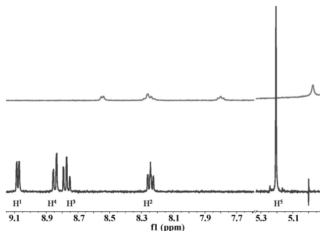
Figure 4. 1 H NMR spectra of G2 (bottom) and of a mixture of equimolar G2 and 8 (top) in D 2 O at 297 K.
